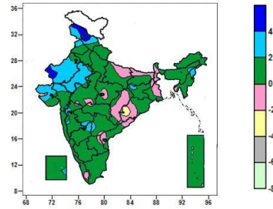
Mean Maximum Temperature (°C) Anomaly in India for the week ending 18.02.2015
