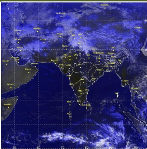
Satellite image dated, 20.02.2015, 0600 UTC
