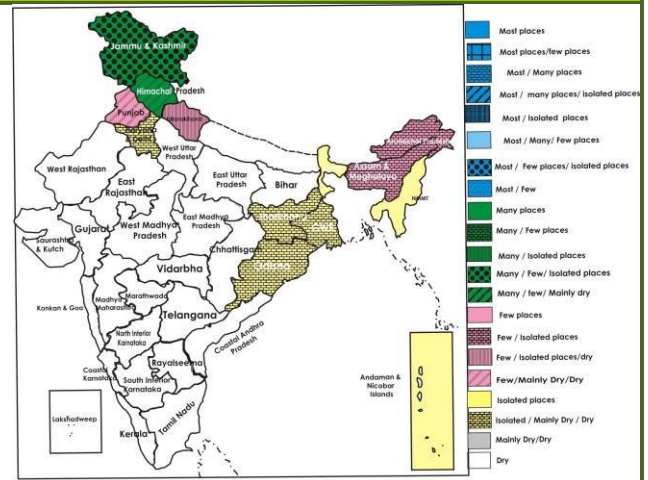
Weather Forecast Map (Valid upto 0830 hours of 23 rd February, 2015)
