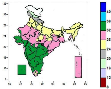
Actual Mean Maximum Temperature (°C) in India for the week ending 18.02.2015
